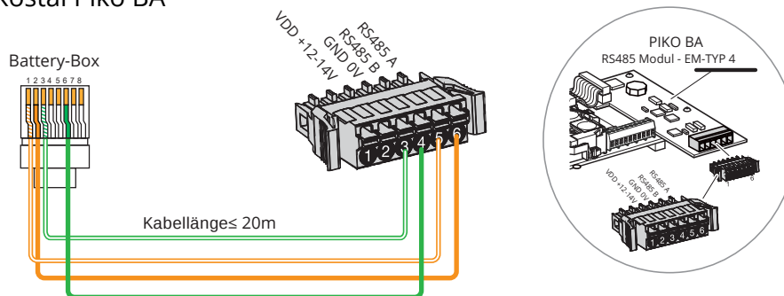
Battery-Box Kostal
