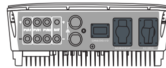
Battery-Box SMA
