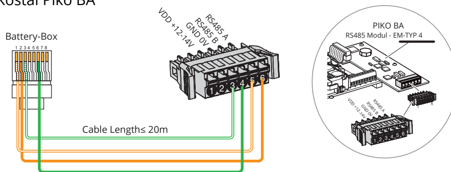
Battery-Box Kostal
